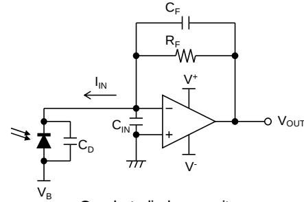
Figure20. Transimpedance amplifier
