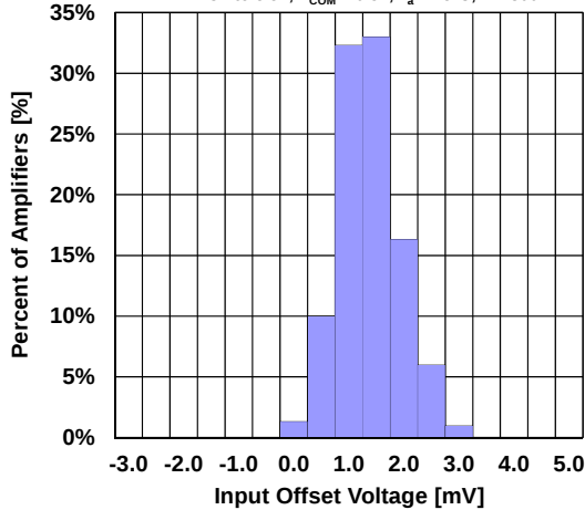
Input Offset Voltage Distribution
