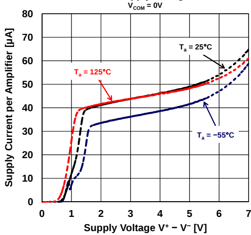
Supply Current per Amplifier vs. Supply Voltage
