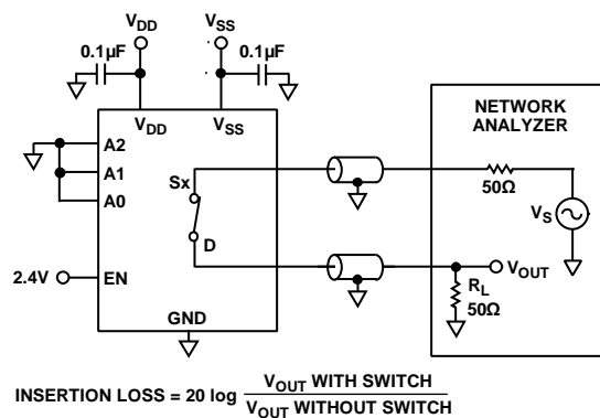
Figure 34. -3 dB Bandwidth
