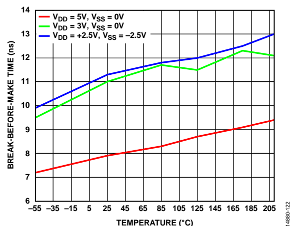
Figure 23. Break-Before-Make Time vs. Temperature
